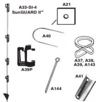
Fiberglass Rod Posts White SunGUARD II™ Coated
